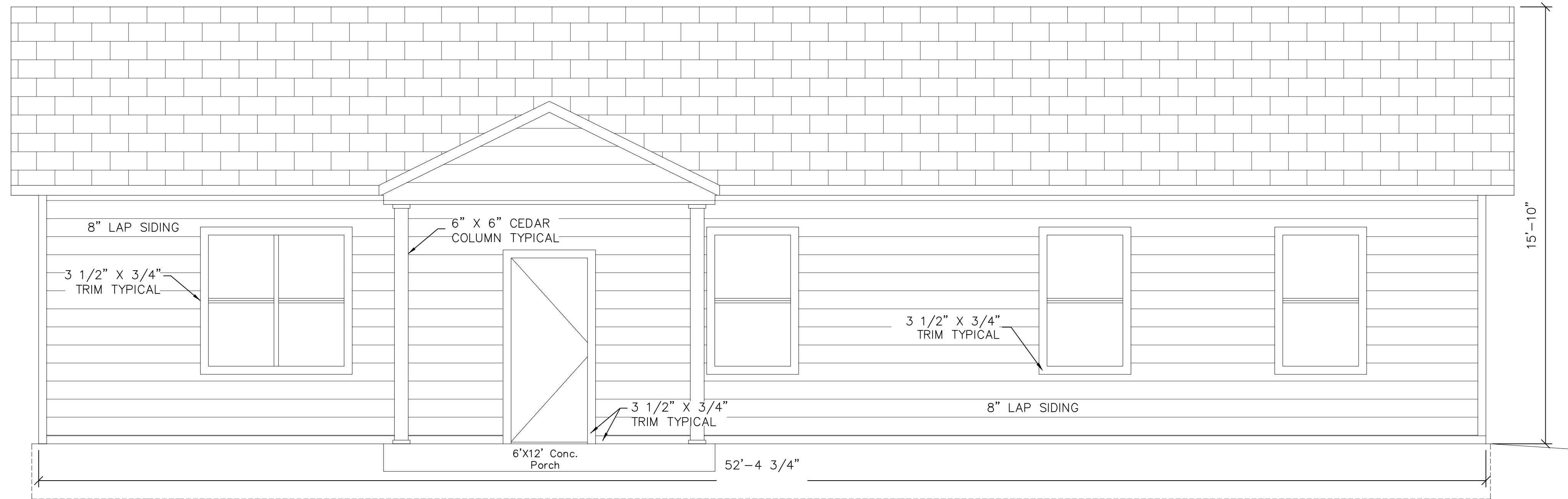
FRONT ELEVATION
