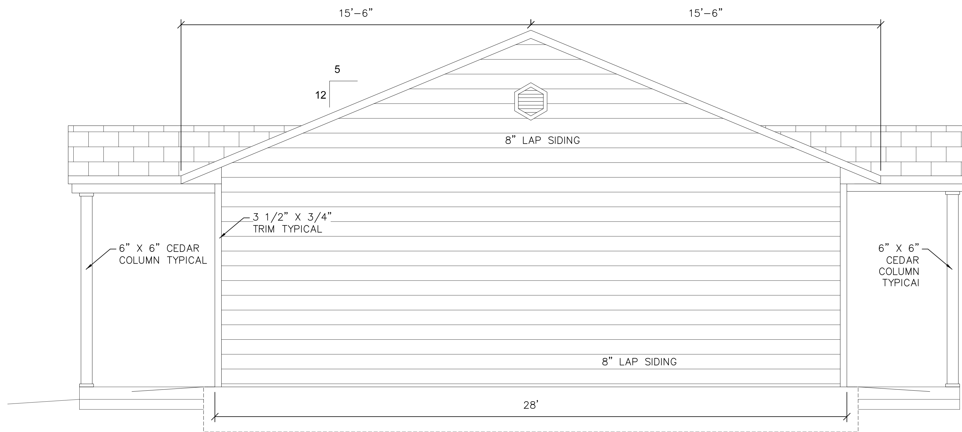
SIDE ELEVATION
