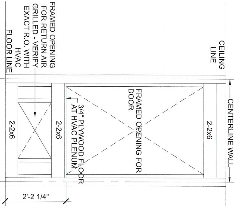
HVAC CLOSET FRAMING SCALE 1"=1/2"=1'
