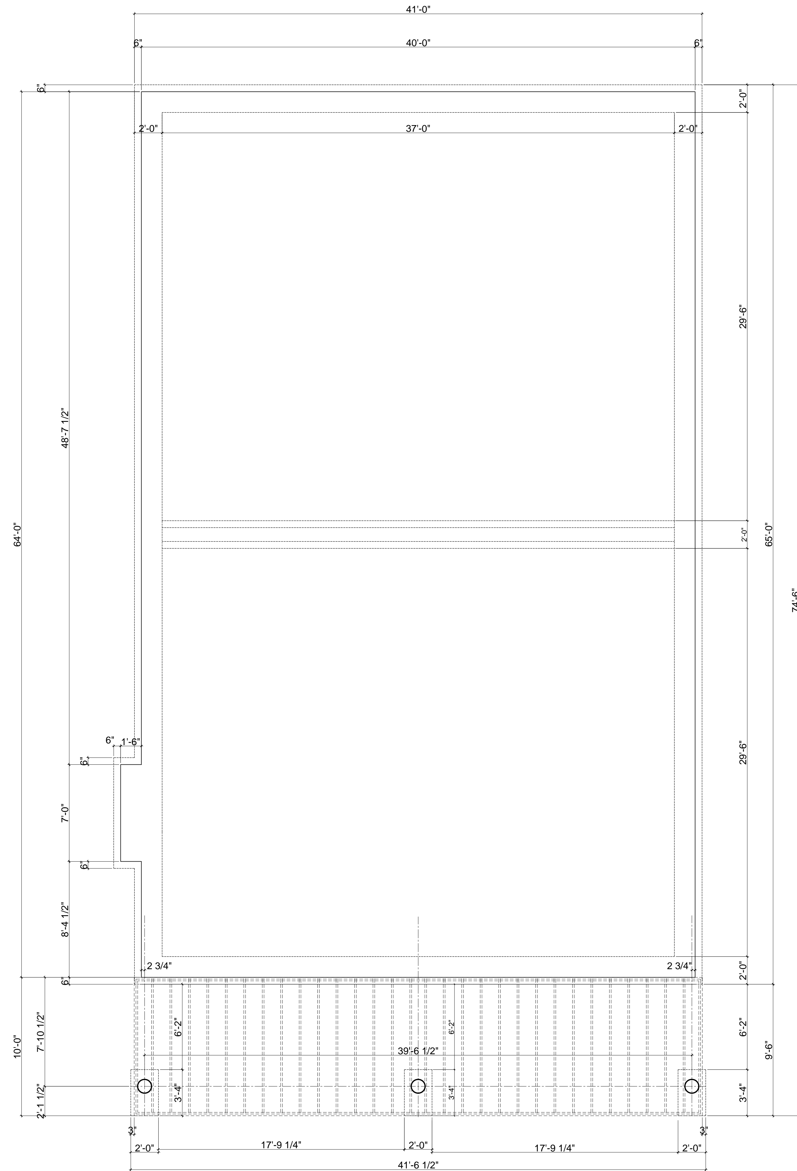
1 6-BED + LOFT CABIN - FOUNDATION PLAN SCALE: 1/4"=1'-0"
