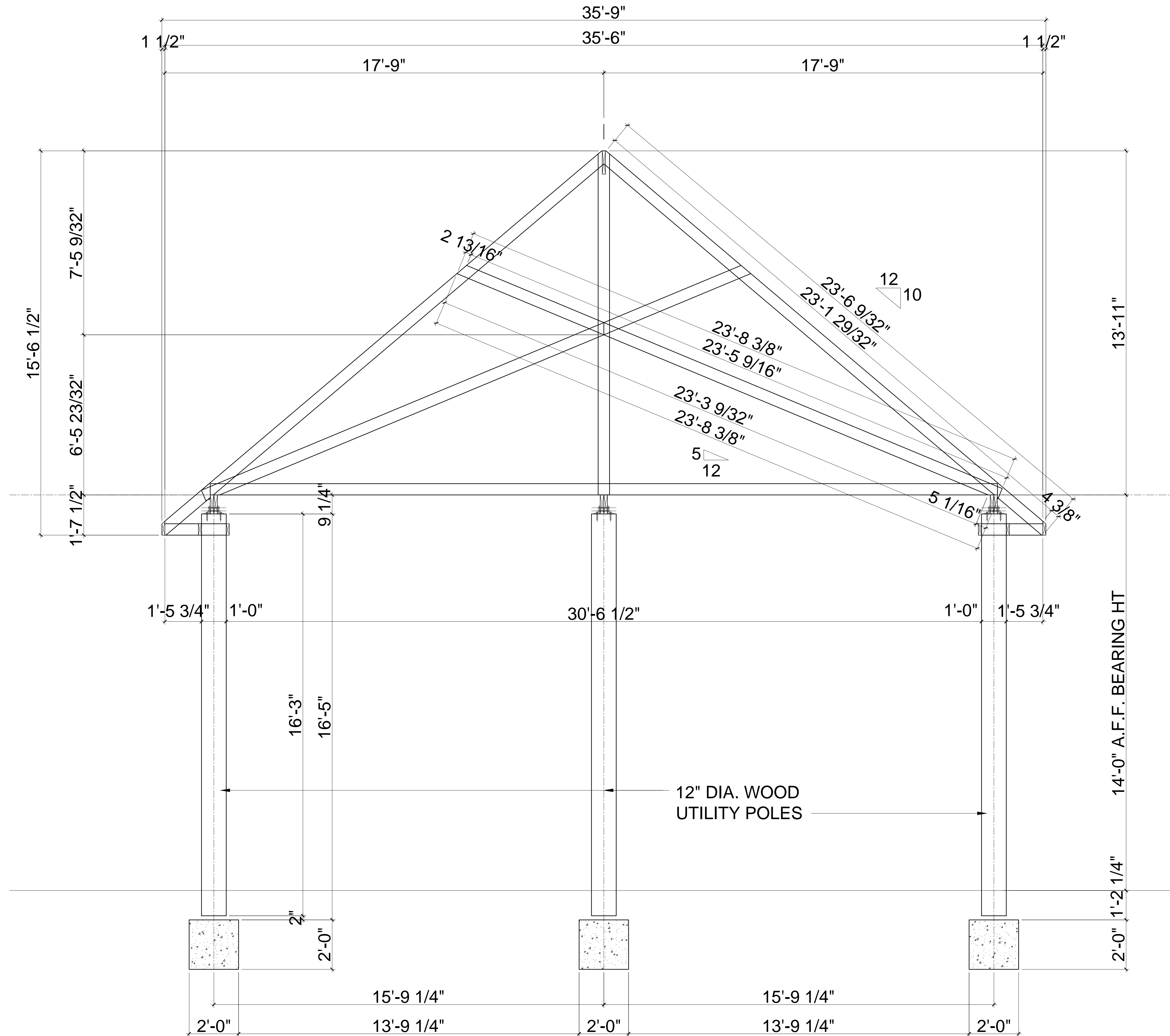
3 4 BED + LOFT SECTION THRU GABLE END ROOF TRUSS SCALE: 1/2"=1'-0"
